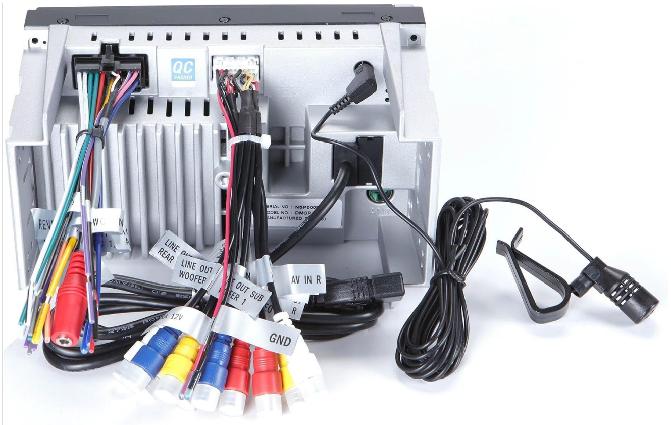
This image displays the included wiring harness and external microphone, essential components for connecting the receiver to your vehicle's electrical system and for hands-free communication.
