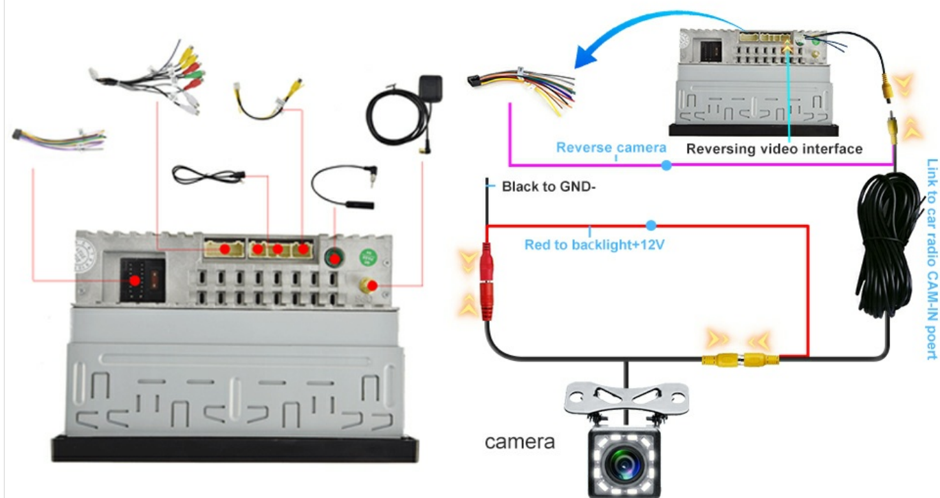
Image: Simplified wiring diagram illustrating connections for power, ground, backlight, and reverse camera input to the car stereo.
