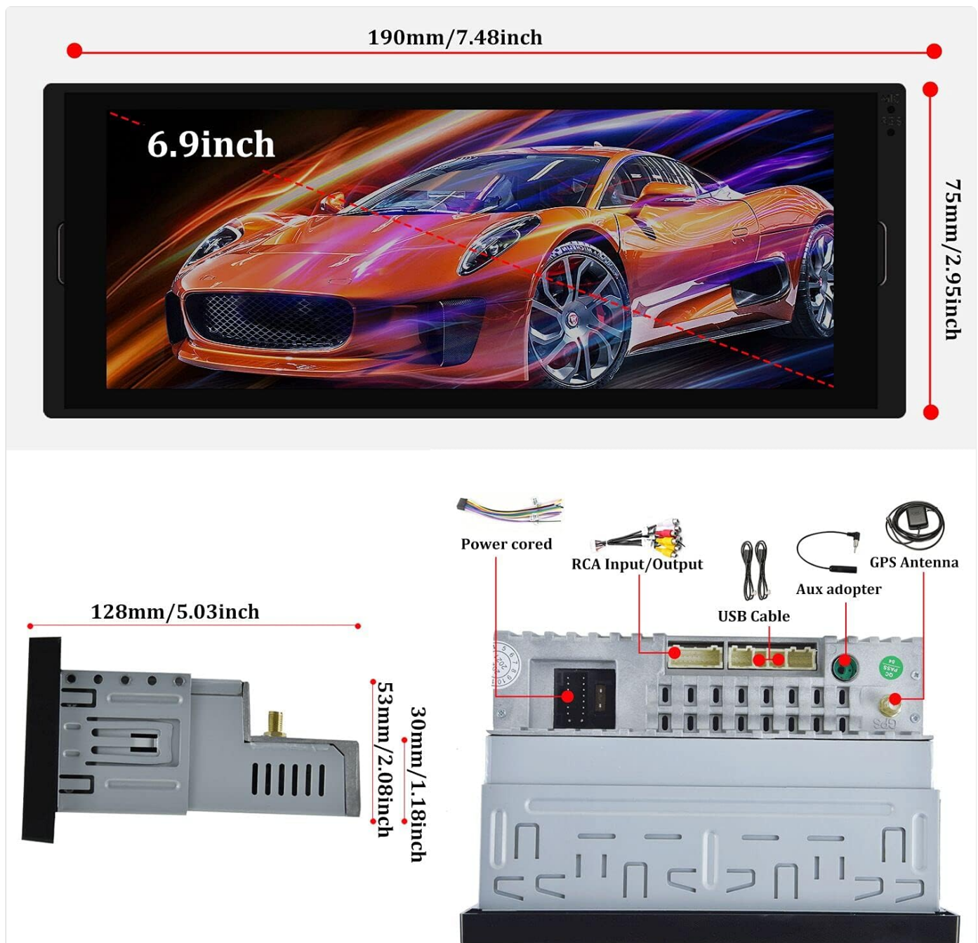
Image: Diagram showing the front and side dimensions of the 6.9-inch car stereo unit, including its depth and width.
