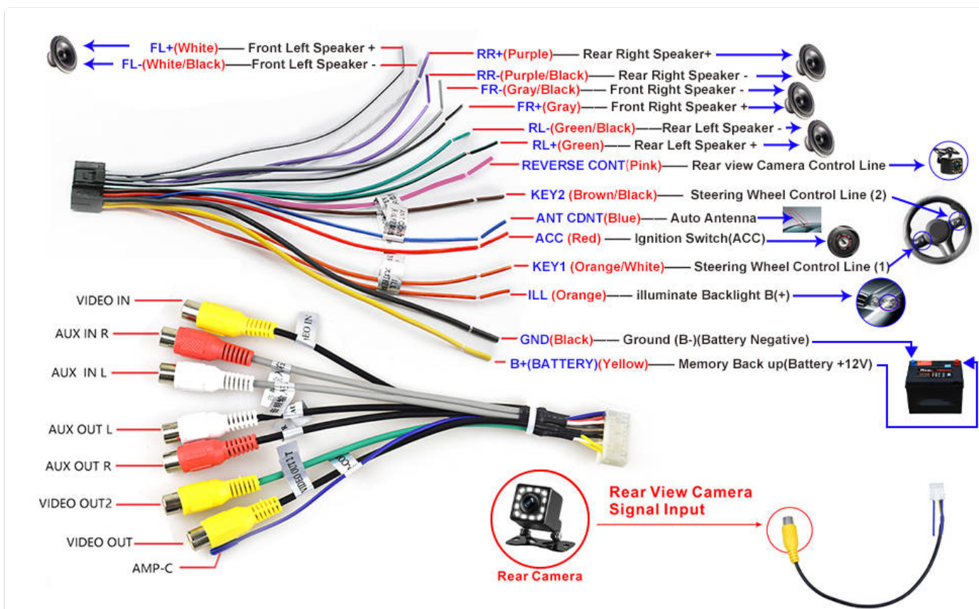
Image: Detailed wiring harness diagram showing connections for front/rear speakers, power (ACC, B+, GND), antenna, steering wheel controls, video inputs/outputs, and reverse camera signal.
