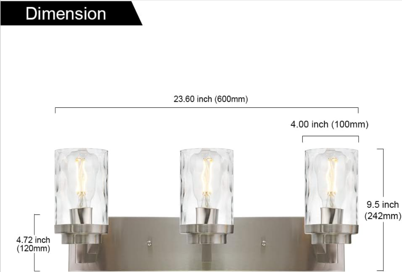
Figure 3: Product Dimensions
