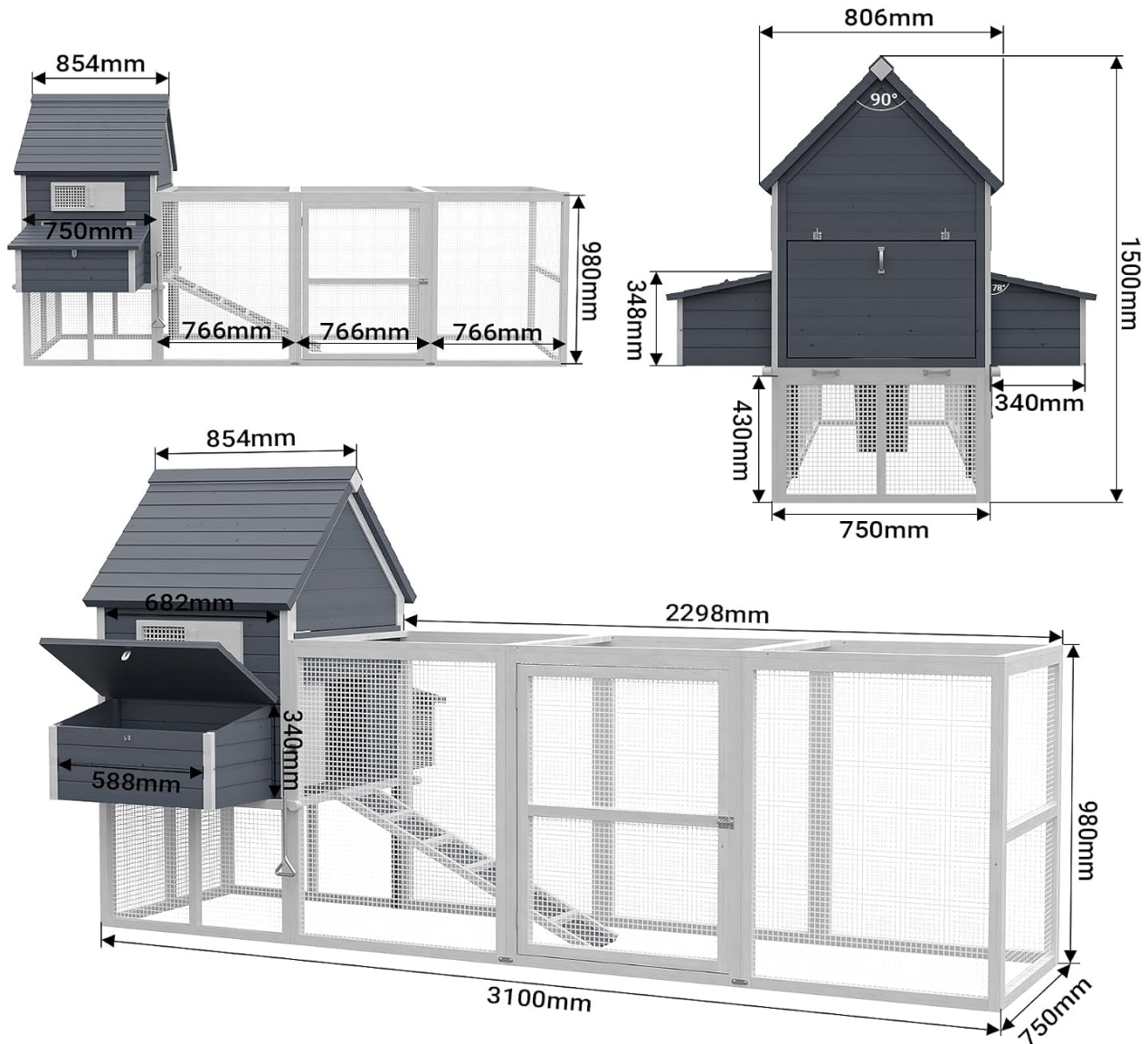
Image: A technical diagram illustrating the various dimensions of the chicken coop, including height, length, and width of different sections.
