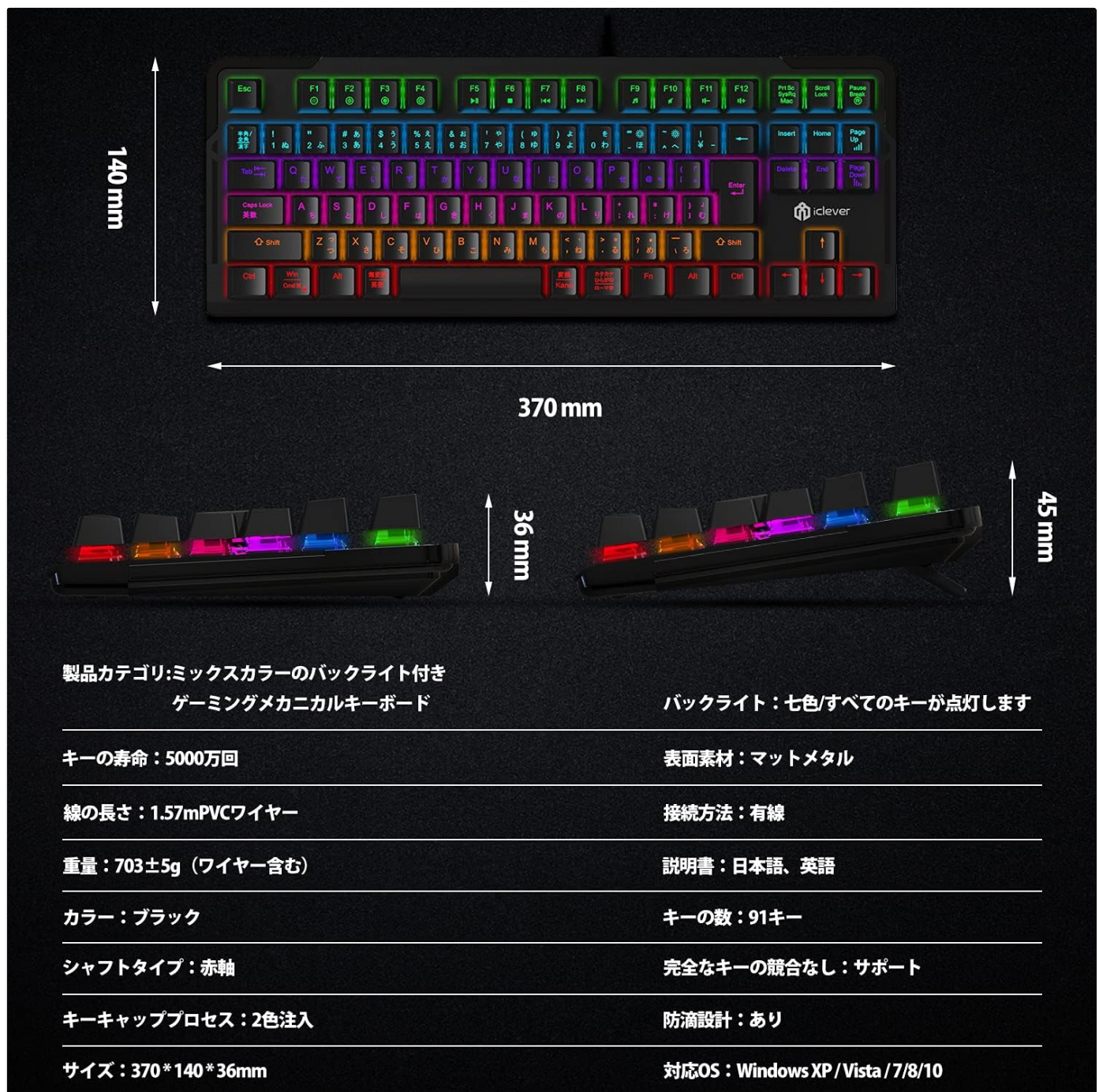
Image 7.1: Keyboard Dimensions and Key Specifications.
