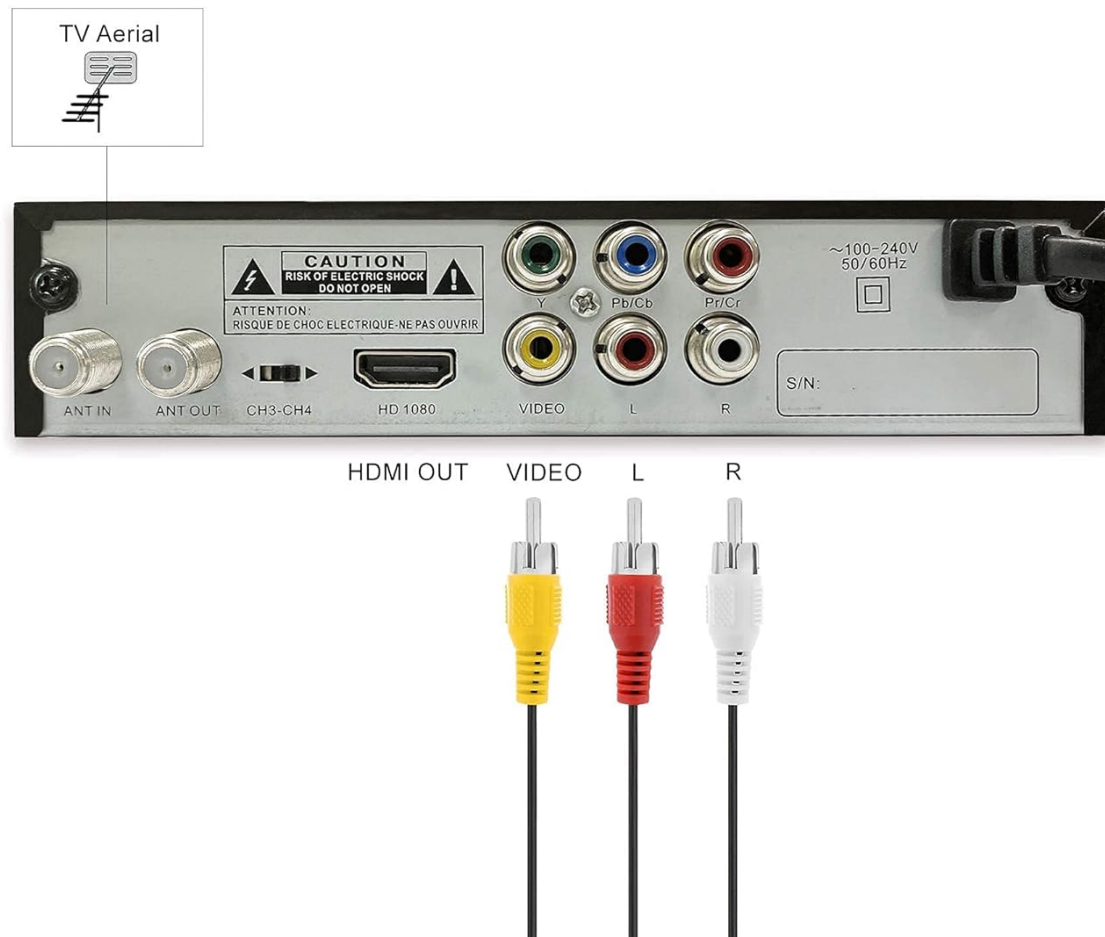
Image: The rear panel of the converter box, showing the antenna input, HDMI output, and RCA audio/video ports.
