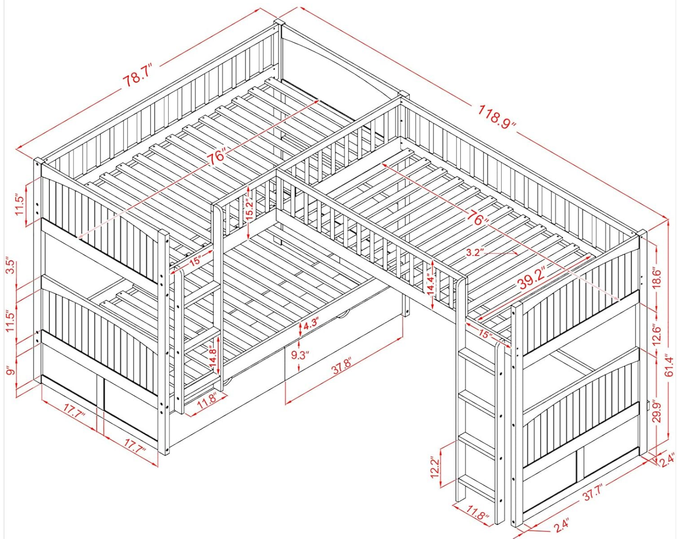
Figure 1: Detailed dimensions of the Bellemave Triple L-Shaped Bunk Bed. This diagram shows the overall length, width, and height, as well as individual bed dimensions and clearances.
