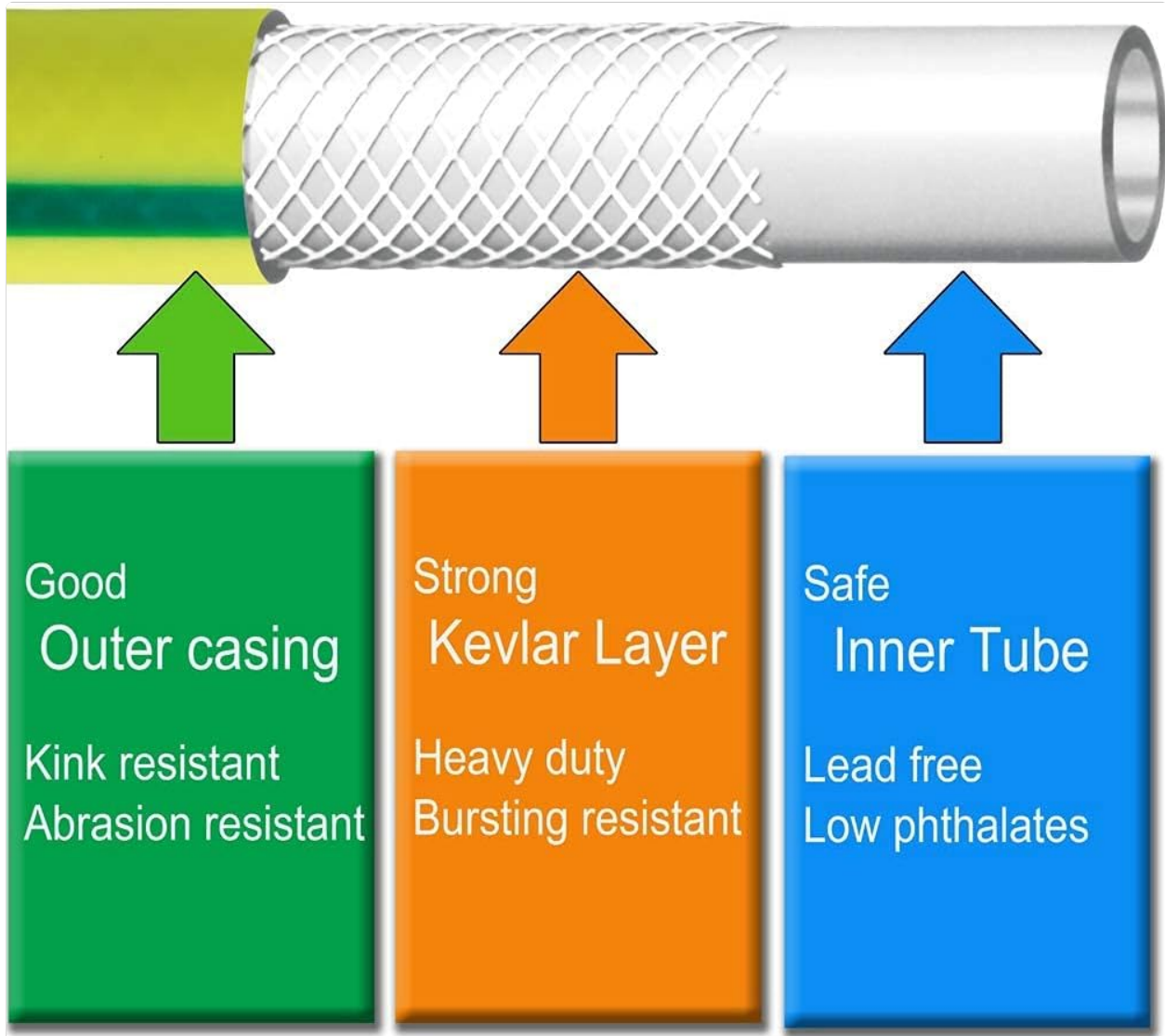
Figure 5: Hose construction with three layers for durability and performance.
