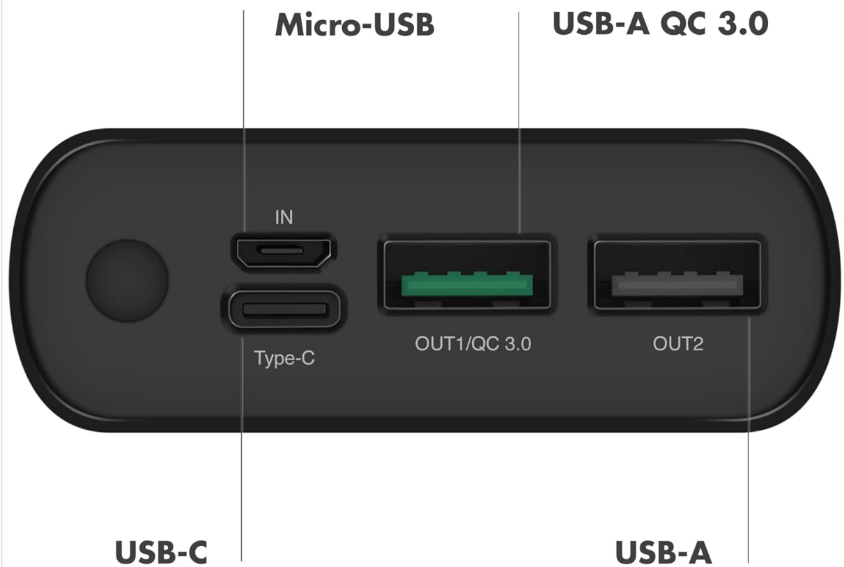
Image 3: A detailed view of the power bank's ports, including Micro-USB (IN), Type-C (IN/OUT), USB-A QC 3.0 (OUT1), and USB-A (OUT2).
