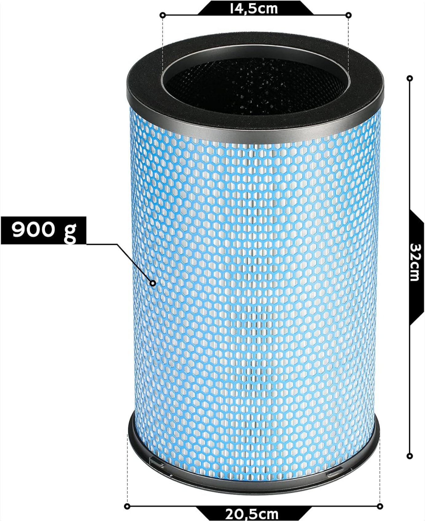
An image of the cylindrical filter with measurements indicating its height (32cm), diameter (20.5cm), and top opening diameter (14.5cm),
