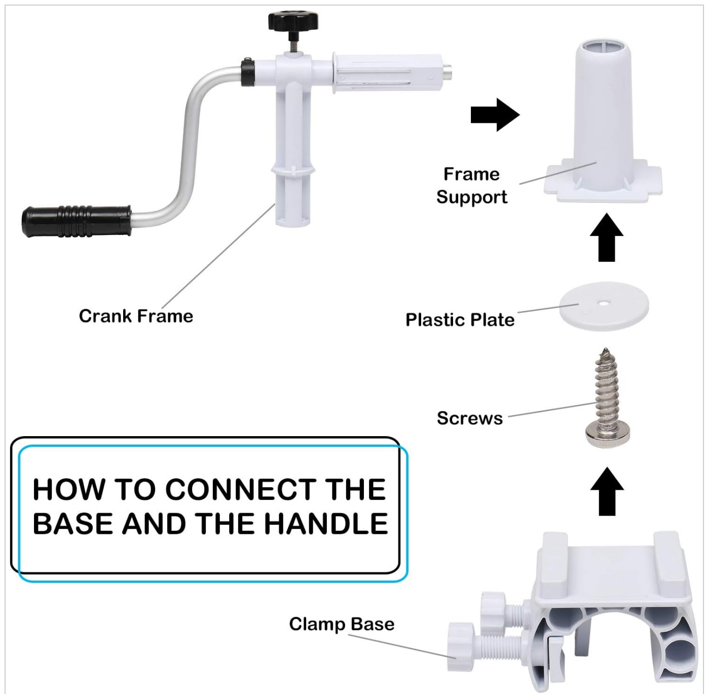
Figure 3.1: Steps for connecting the base and handle components.
