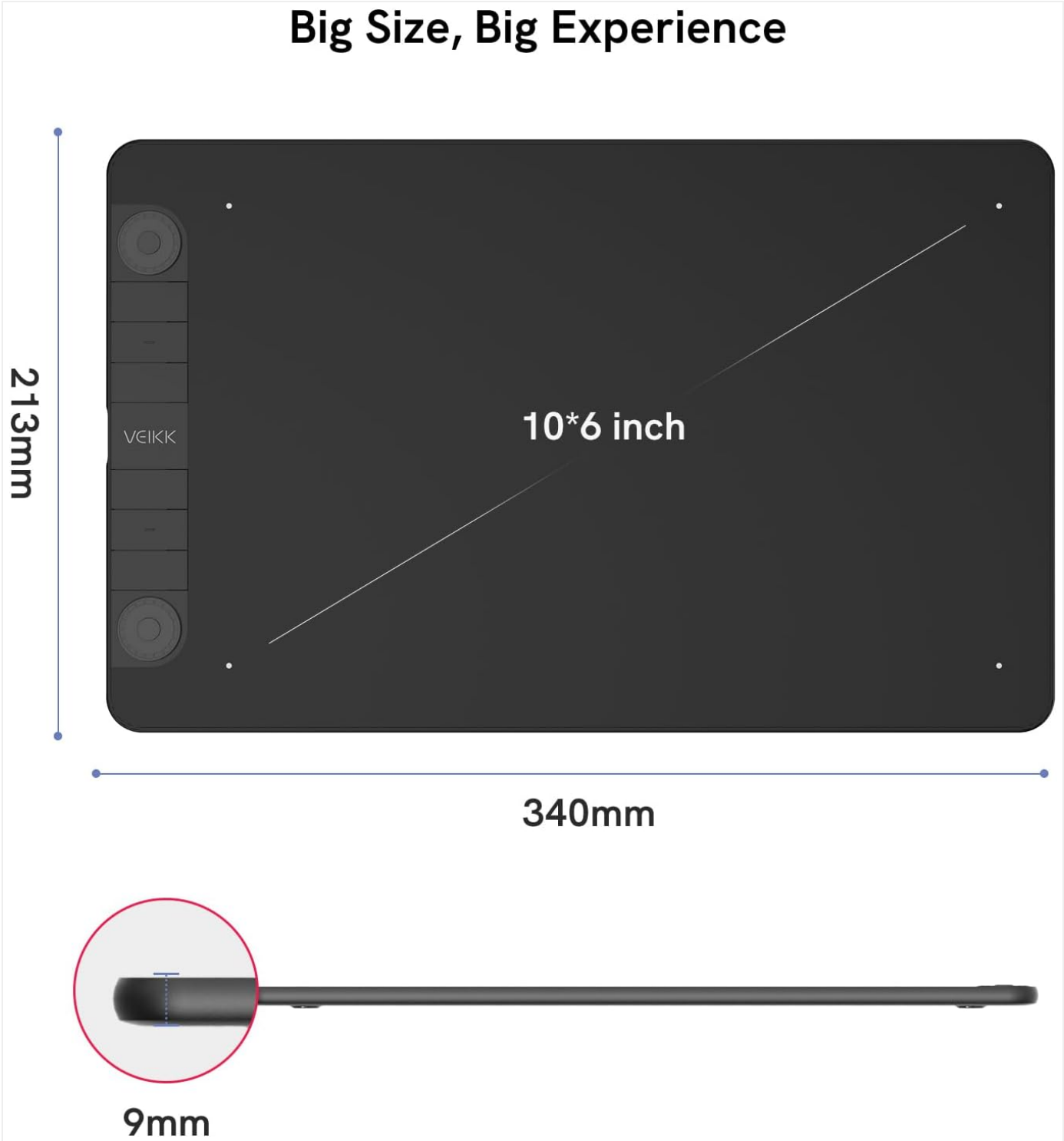
Image: Visual representation of the VEIKK VK1060PRO V2 tablet's dimensions, highlighting its 10x6 inch active area and slim 9mm profile.
