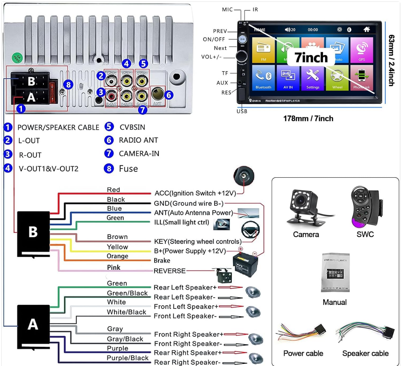
Figure 4.2: Comprehensive wiring diagram illustrating connections for power, speakers, camera input, and other peripheral devices. Ensure all connections match the vehicle's wiring system.
