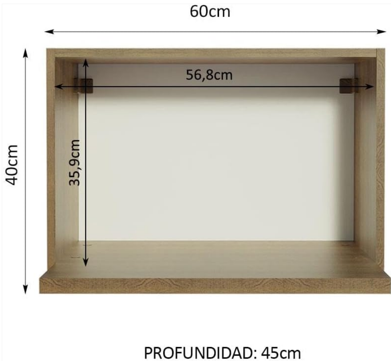
Front view of the Madesa 60cm Oven Cabinet.
