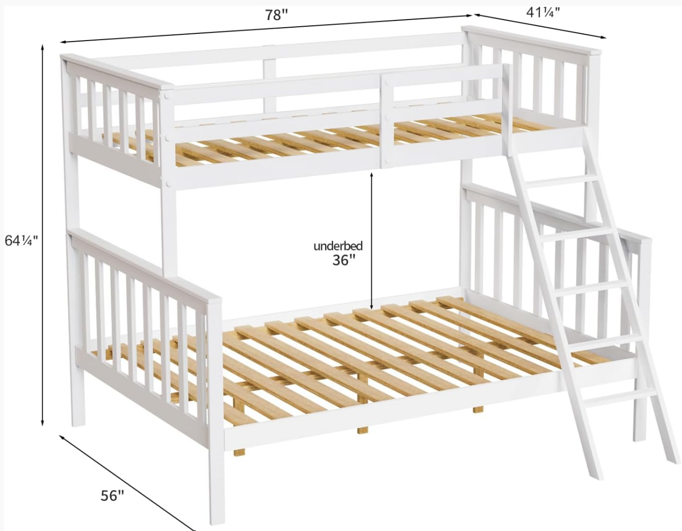
Image 3.1: Dimensional diagram of the JOYMOR Twin Over Full Bunk Bed.
