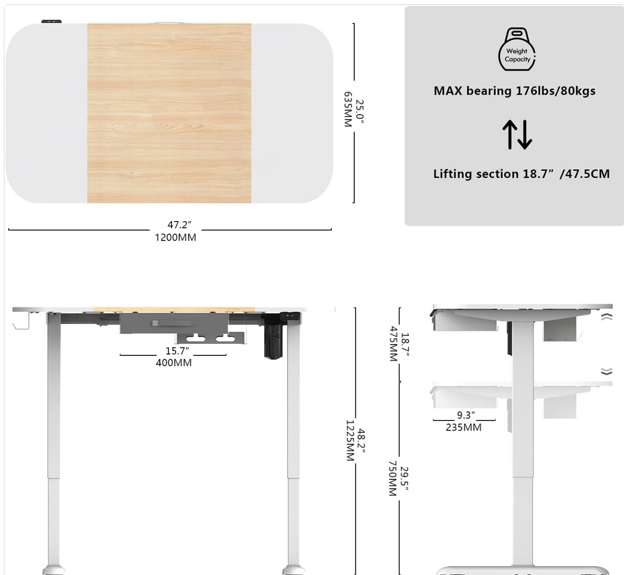
Image: Technical drawing illustrating the desk's dimensions and maximum weight capacity.
