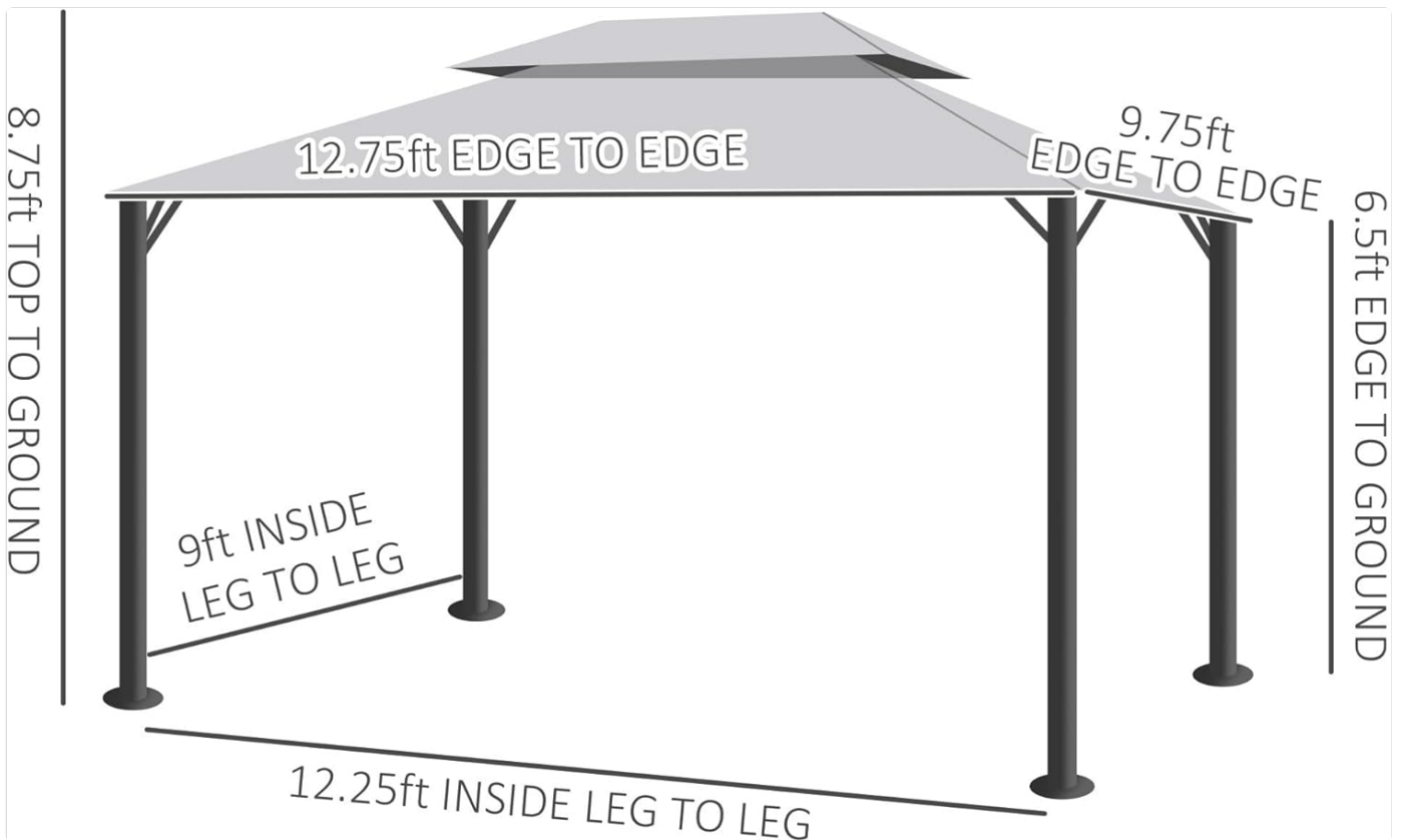
Image: Diagram illustrating the key dimensions of the Outsunny Patio Gazebo, including edge-to-edge and leg-to-leg measurements.
