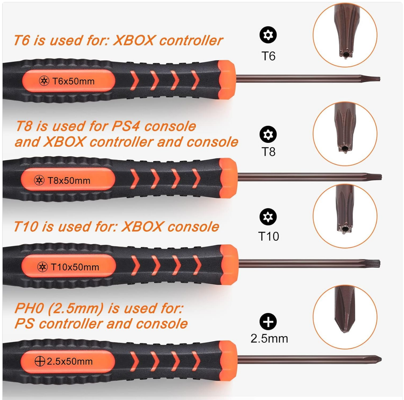
Figure 2: Screwdriver types and their applications.
