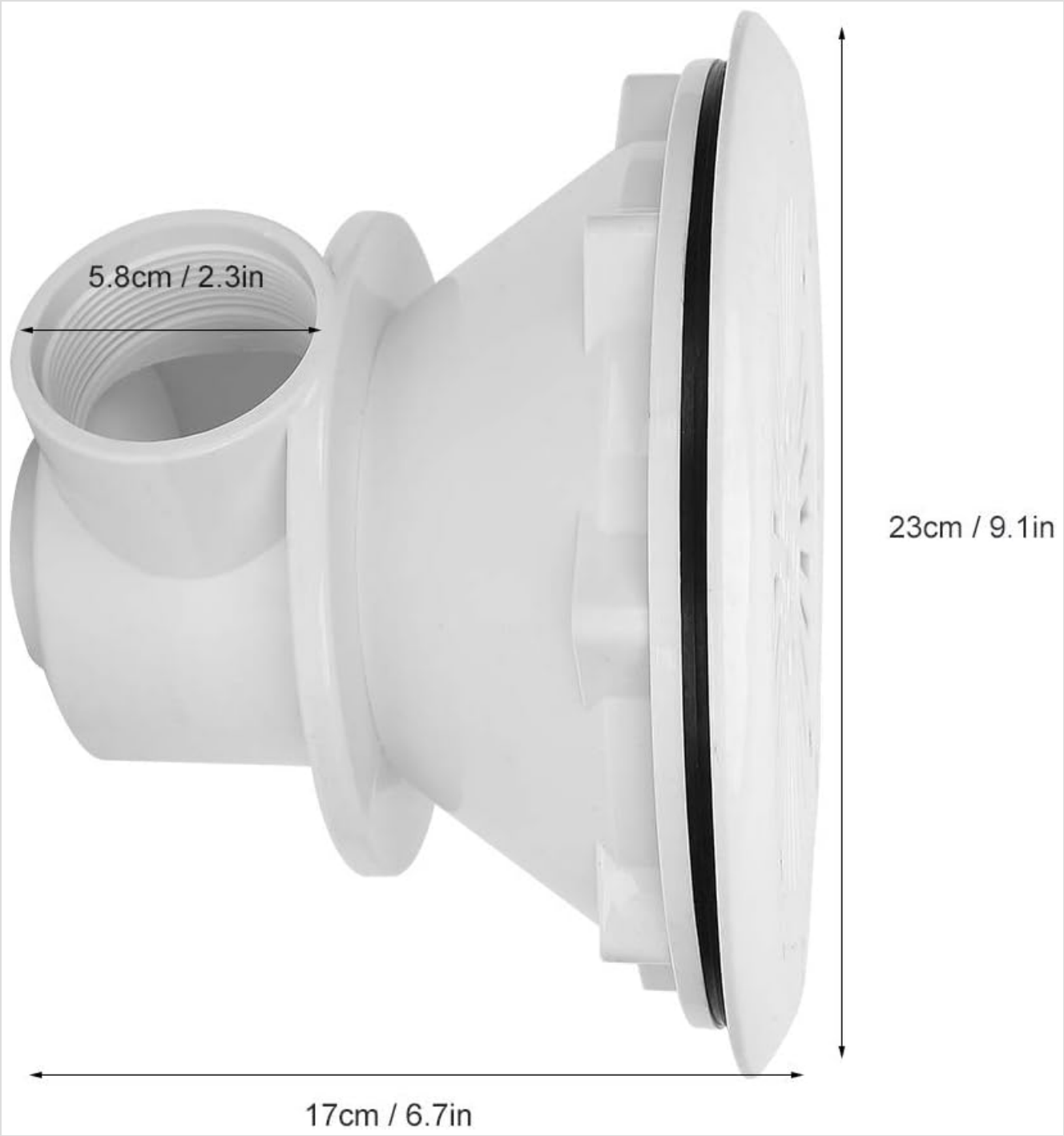
Image 3.1: Dimensional drawing of the pool drain port, indicating key measurements.
