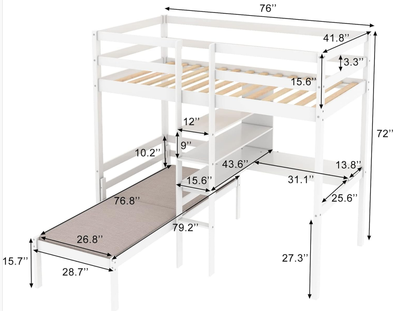
Image: A detailed diagram illustrating the precise dimensions of the Flieks bunk bed in inches, including length, width, and height of various components such as the bunks, desk, and trundle. This provides essential measurements for space planning.
