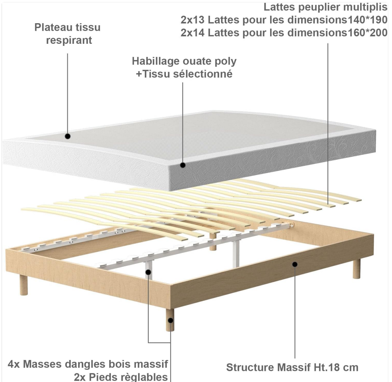
Figure 3.1: Exploded view of the DEWINNER Bed Base components, showing the frame, slats, and various leg types.
