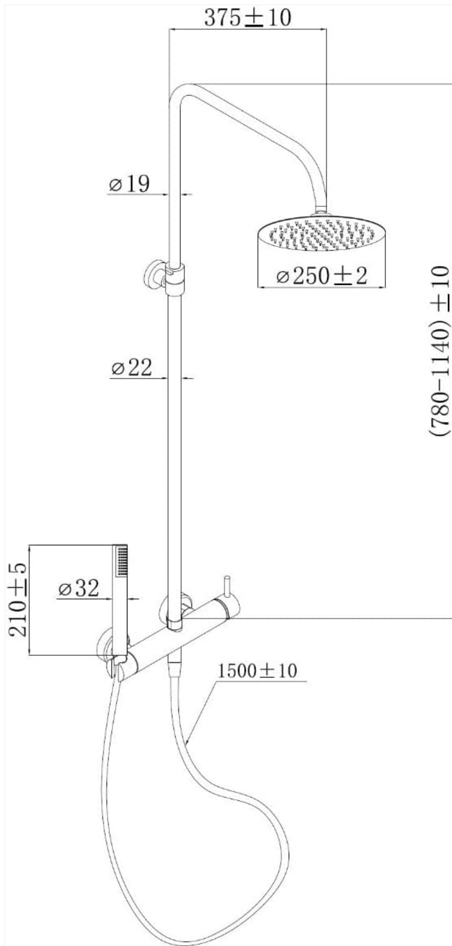
Figure 1: Technical diagram showing the dimensions and components of the shower column.
