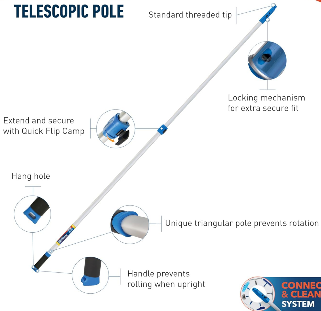
Figure 4: Features of the 8-foot Connect & Clean Telescopic Pole.
