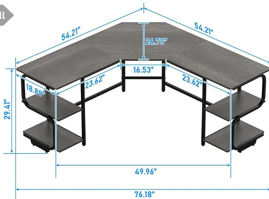
Figure 4.1: Reference desk dimensions during assembly.
