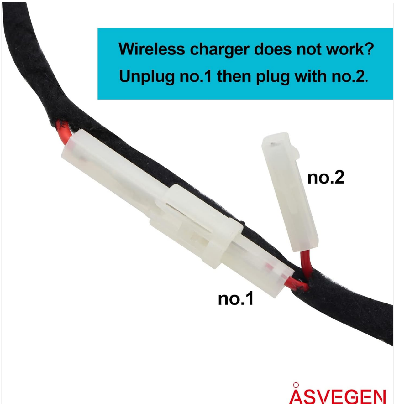
Figure 5: Power Connection Troubleshooting
