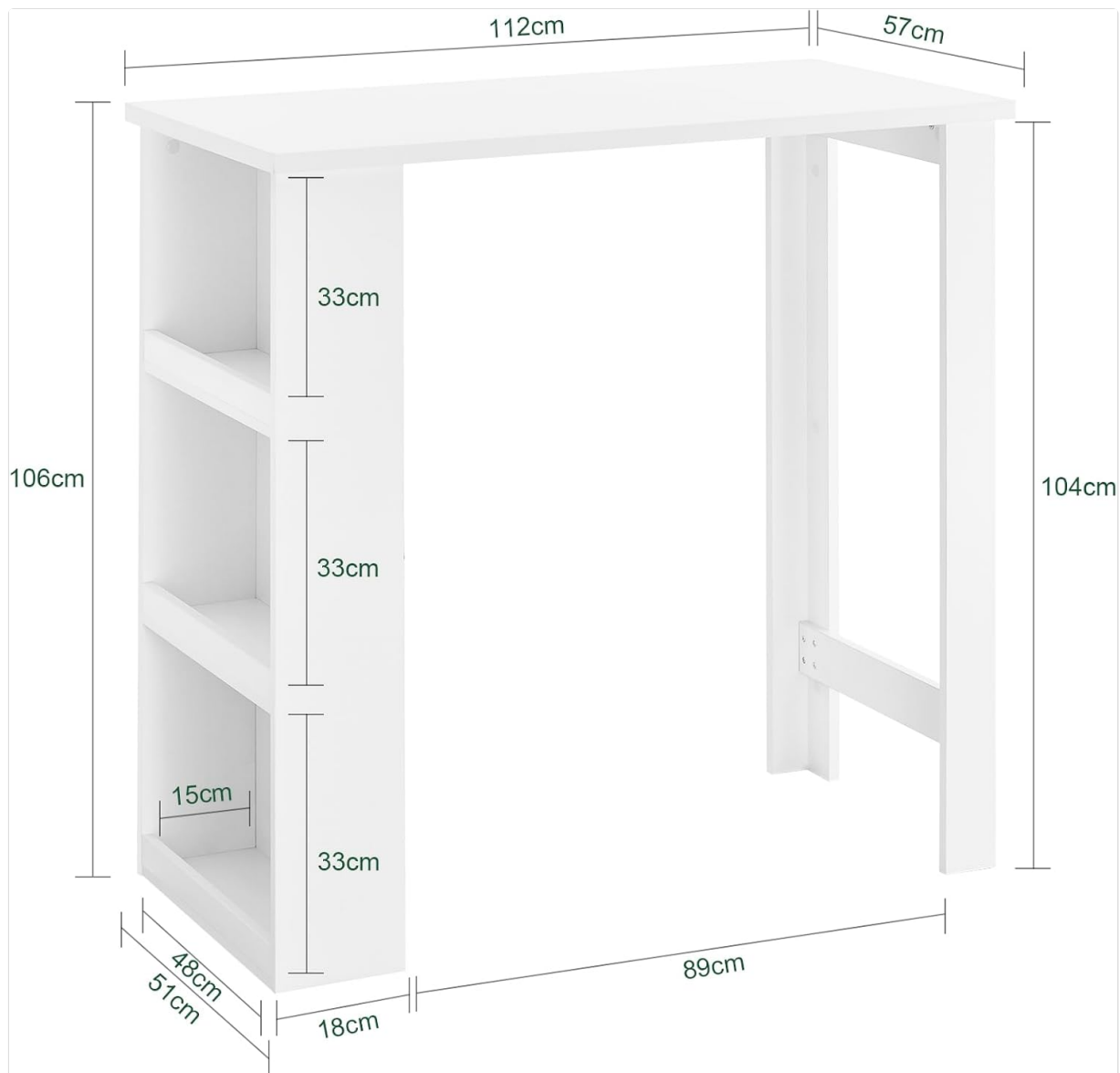
Image 2.2: Technical drawing displaying the overall dimensions of the bar table, including height, width, depth, and shelf spacing.
