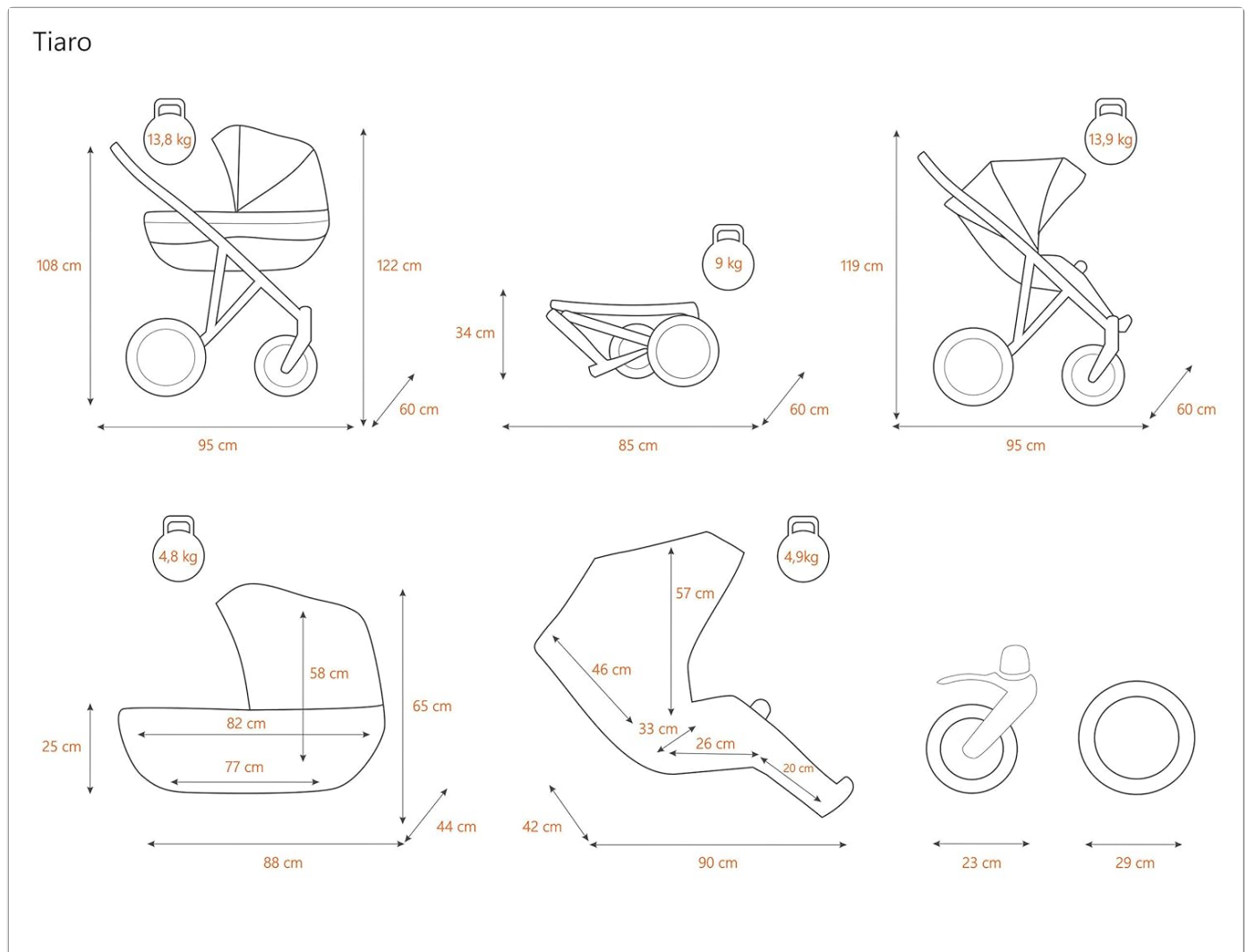
Image 7.1: Detailed technical diagram illustrating the dimensions and weights of the Kunert Tiaro stroller in different configurations (bassinet, seat, folded).
