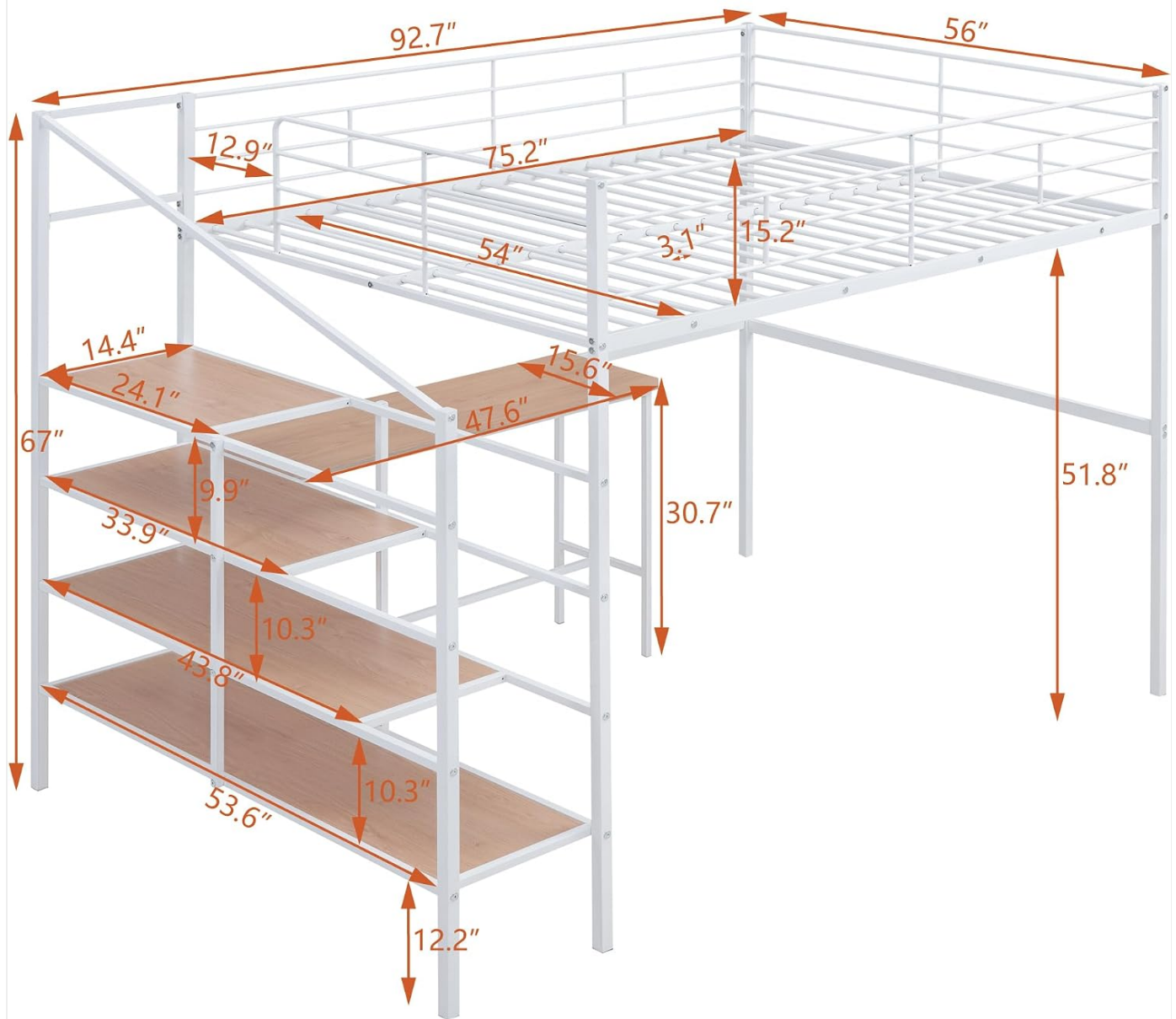
Image 8.1: Detailed diagram illustrating the dimensions of the SOFTSEA Full Size Loft Bed, including length, width, height, and specific measurements for the bed area, desk, and staircase shelves.
