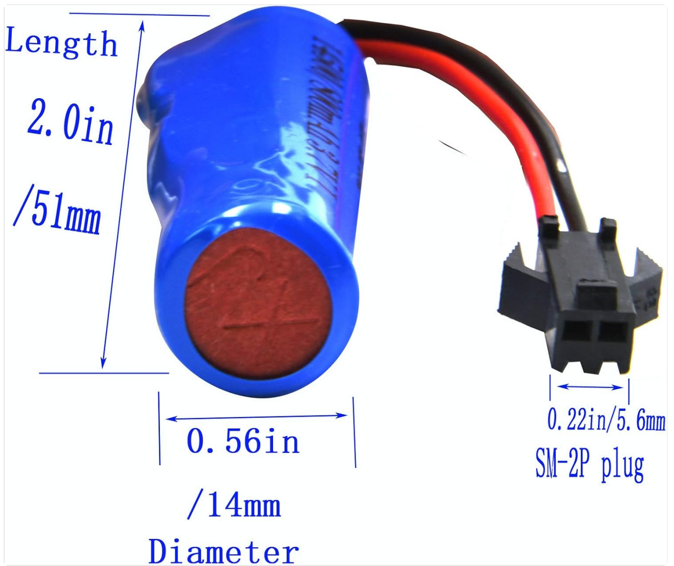
Image: Detailed dimensions of the Blomiky 3.7V Li-ion battery and its SM-2P plug.
