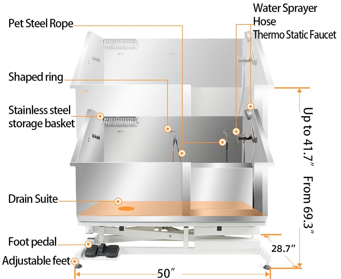
Figure 2: Detailed diagram illustrating the dimensions and key components such as the water sprayer, thermo static faucet, pet steel rope, shaped ring, stainless steel storage basket, drain suite, foot pedal, and adjustable feet.
