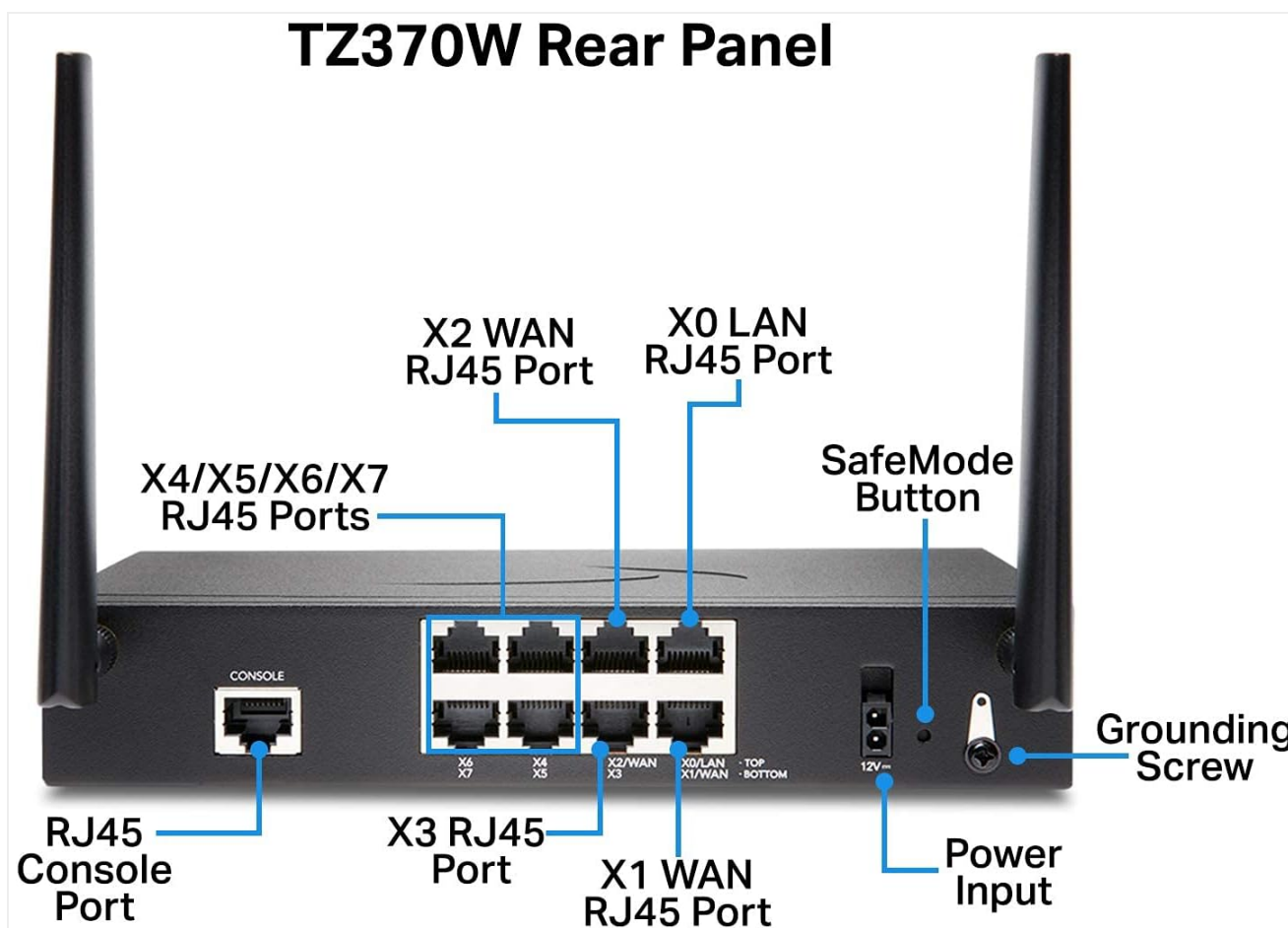
Figure 2.3.2: Labeled Rear Panel of TZ370W. This detailed view identifies the RJ45 Console Port, X3 RJ45 Port, X4/X5/X6/X7
