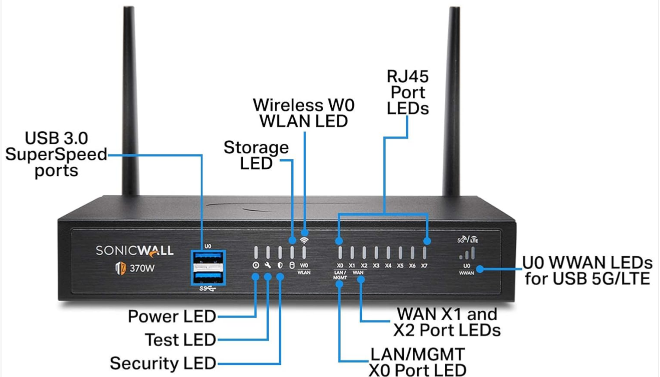
Figure 2.2.1: Sonicwall TZ370W Front Panel. This image displays the front view of the Sonicwall TZ370W Wireless Network Security Appliance, showing the status LEDs, USB 3.0 SuperSpeed ports, and the Sonicwall logo.
