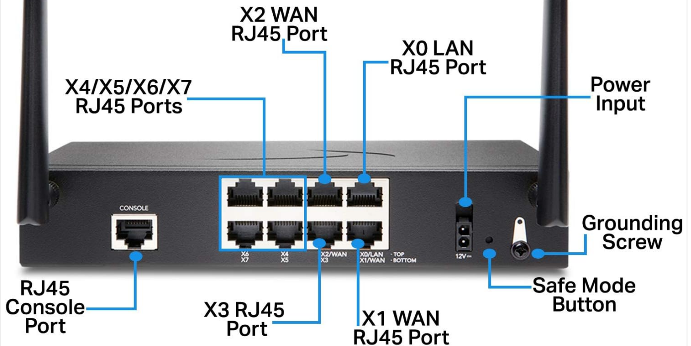
Figure 3: TZ270W Rear Panel Layout
