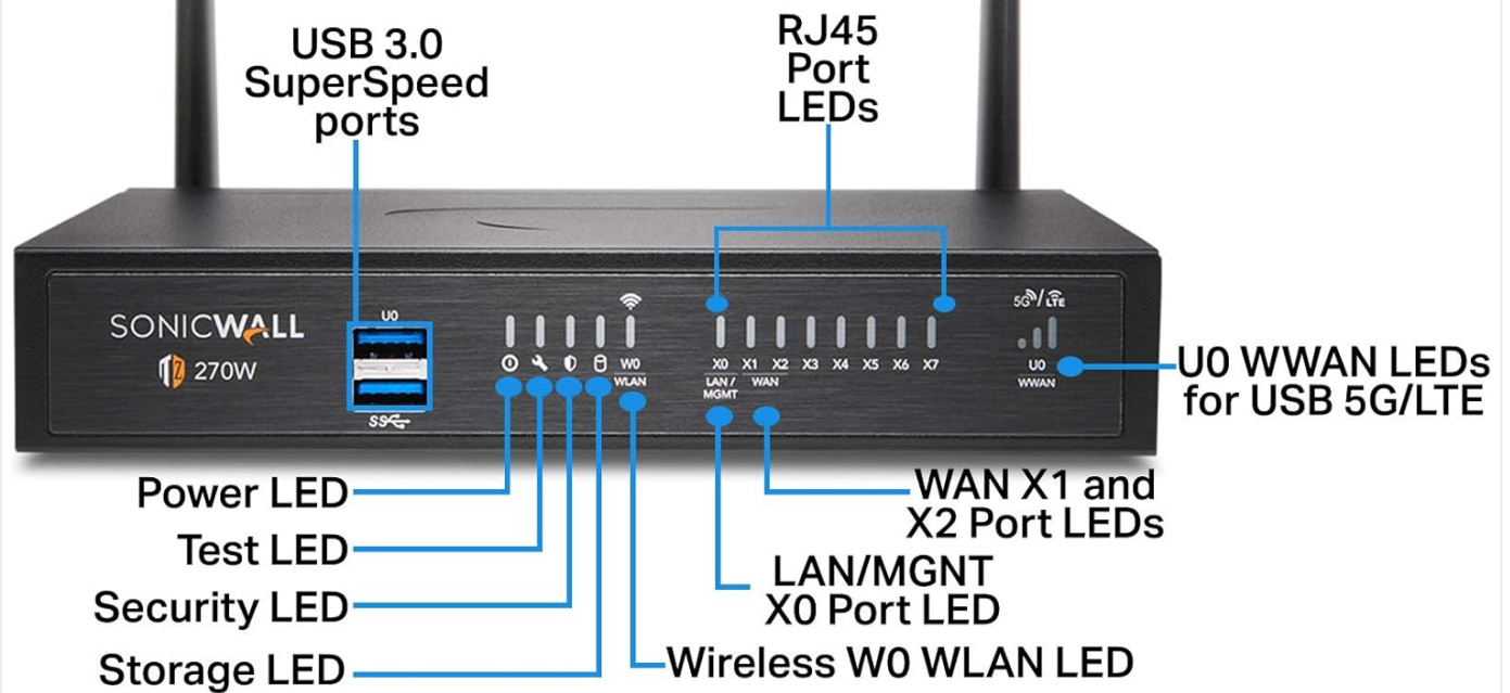
Figure 2: TZ270W Front Panel Layout
