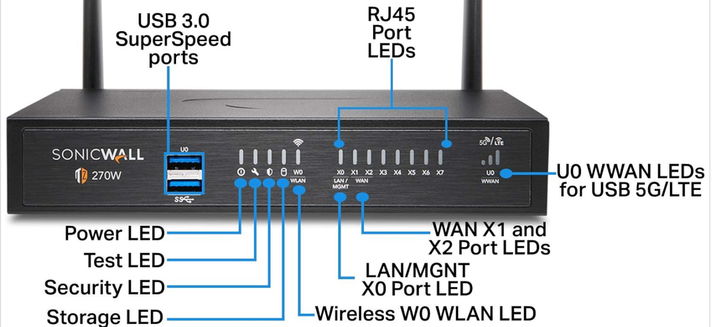
Figure 4.2: Labeled front panel of the TZ270W, highlighting USB 3.0 SuperSpeed ports, RJ45 Port LEDs, Power LED, Test LED, Security LED, Storage LED, Wireless W0 WLAN LED, WAN X1 and X2 Port LEDs, LAN/MGMT X0 Port LED, and U0 WWAN LEDs for USB 5G/LTE.
