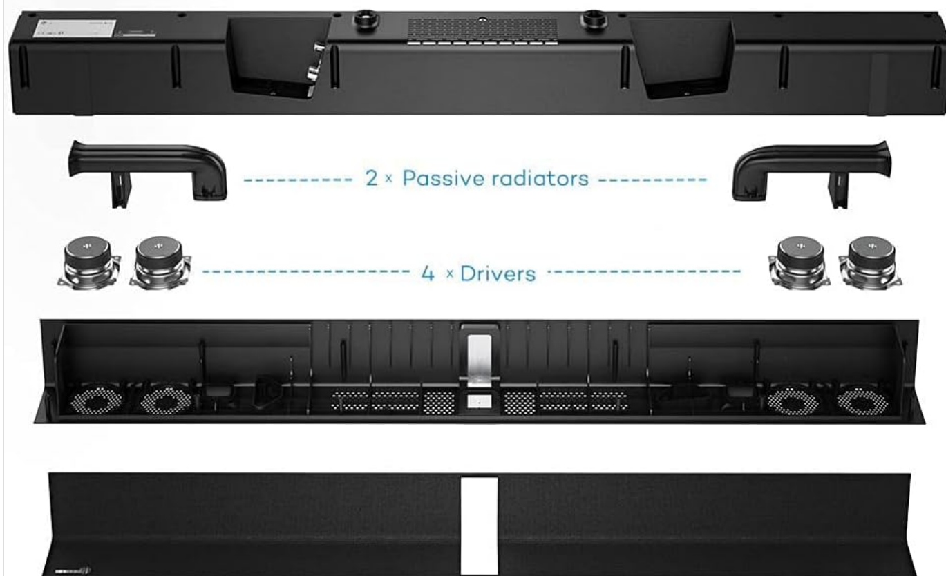
Figure 6: An exploded view of the TT-SK15 Sound Bar, illustrating its internal components including four drivers and two passive radiators, which contribute to its powerful stereo audio output.
