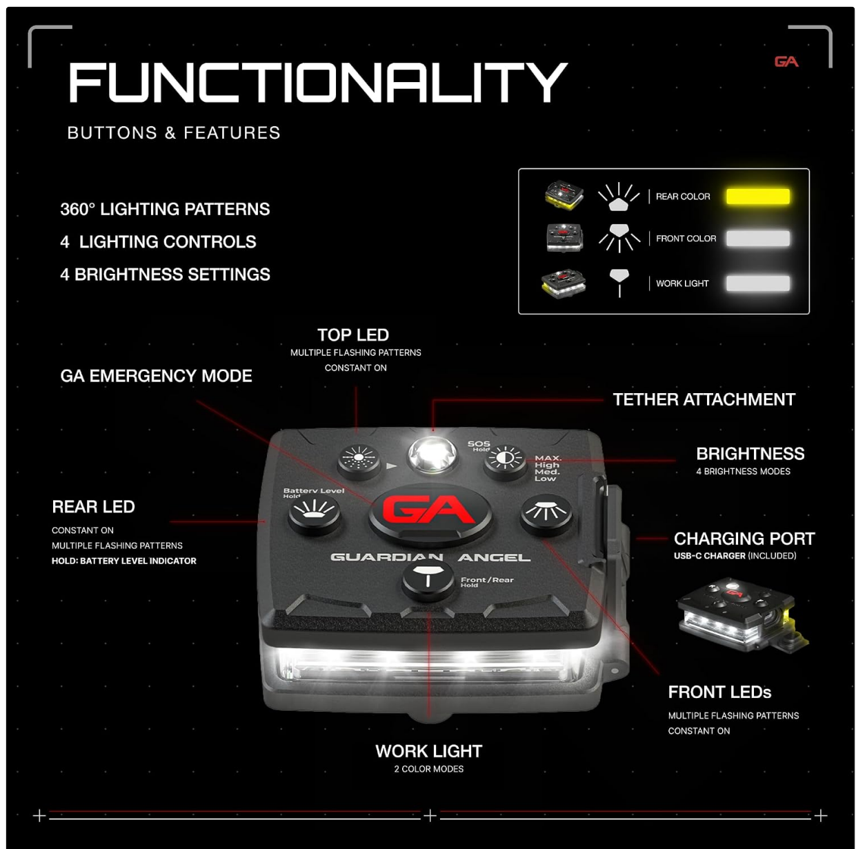
Image 4.1: Overview of the device's buttons and features.
