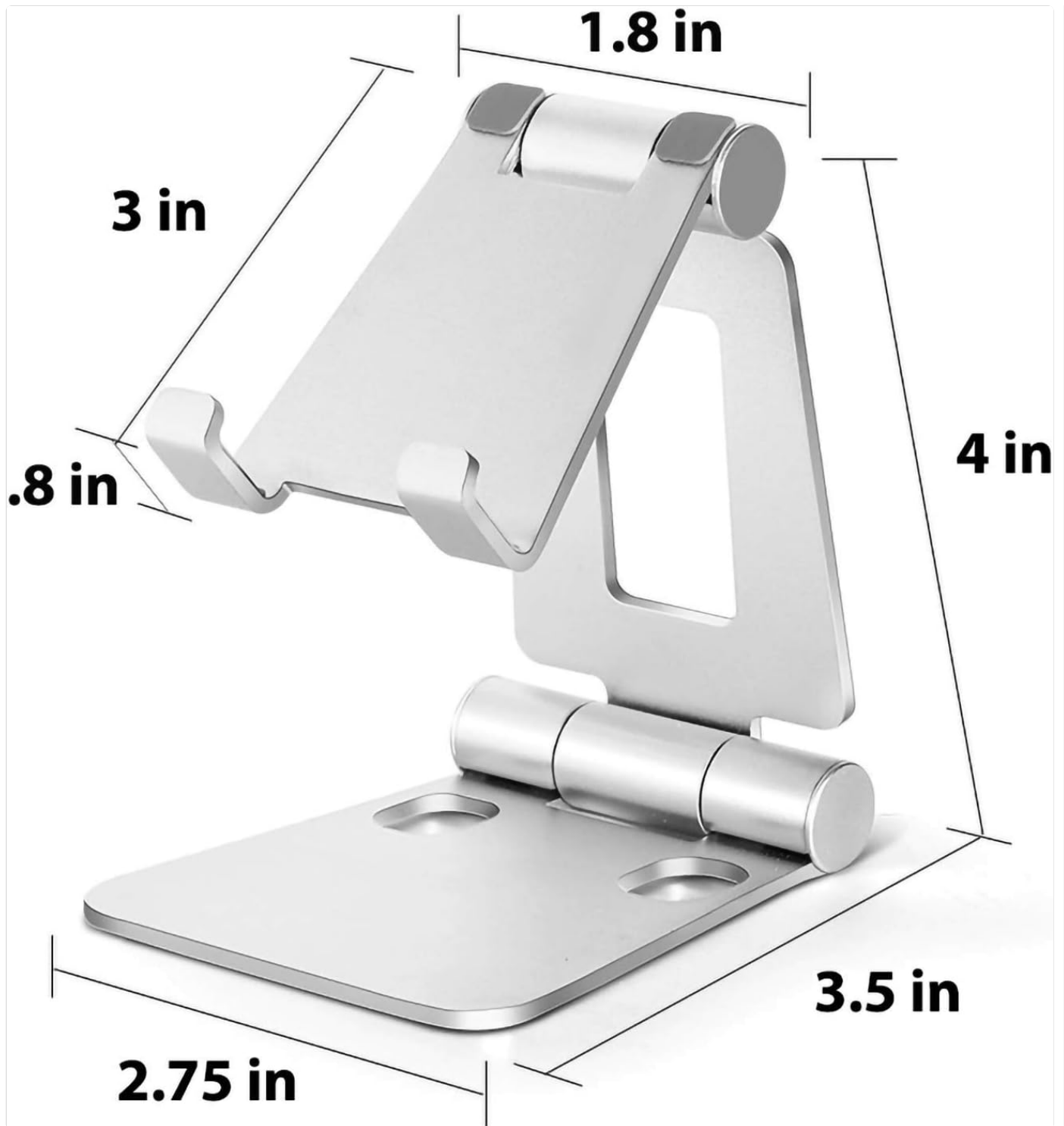
Image 7.1: Detailed dimensions of the PRO Viewing Stand in its open configuration.
