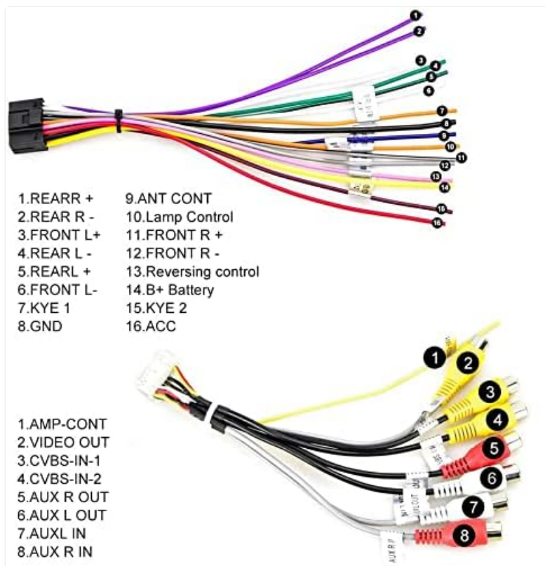
Figure 3: Main wiring harness connections.
