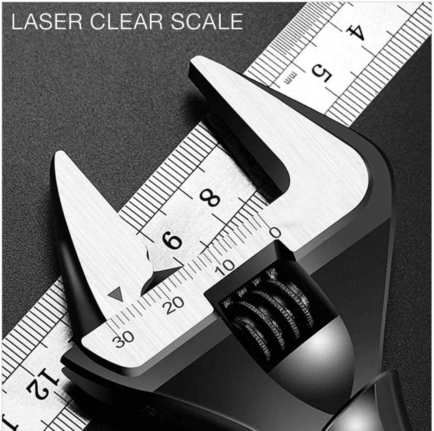
Image: A close-up view of the wrench jaw, highlighting the laser-etched clear scale for precise measurement and adjustment of the jaw opening.
