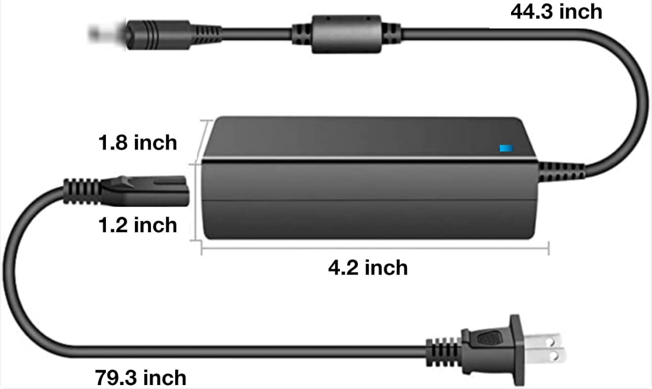
Figure 6.1: Detailed dimensions of the adapter and its cables.
