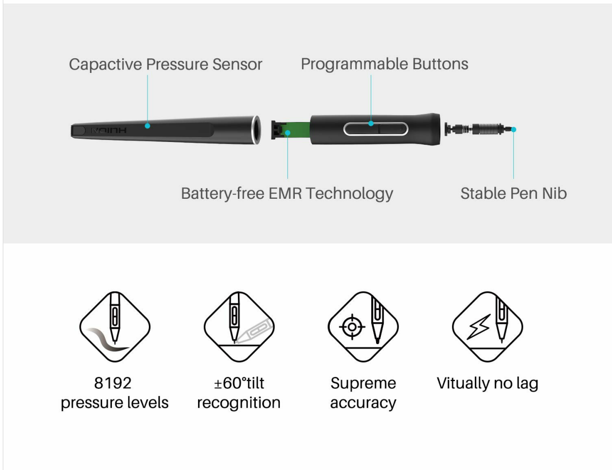
Image 5: Internal components and features of the PW517 digital pen.
