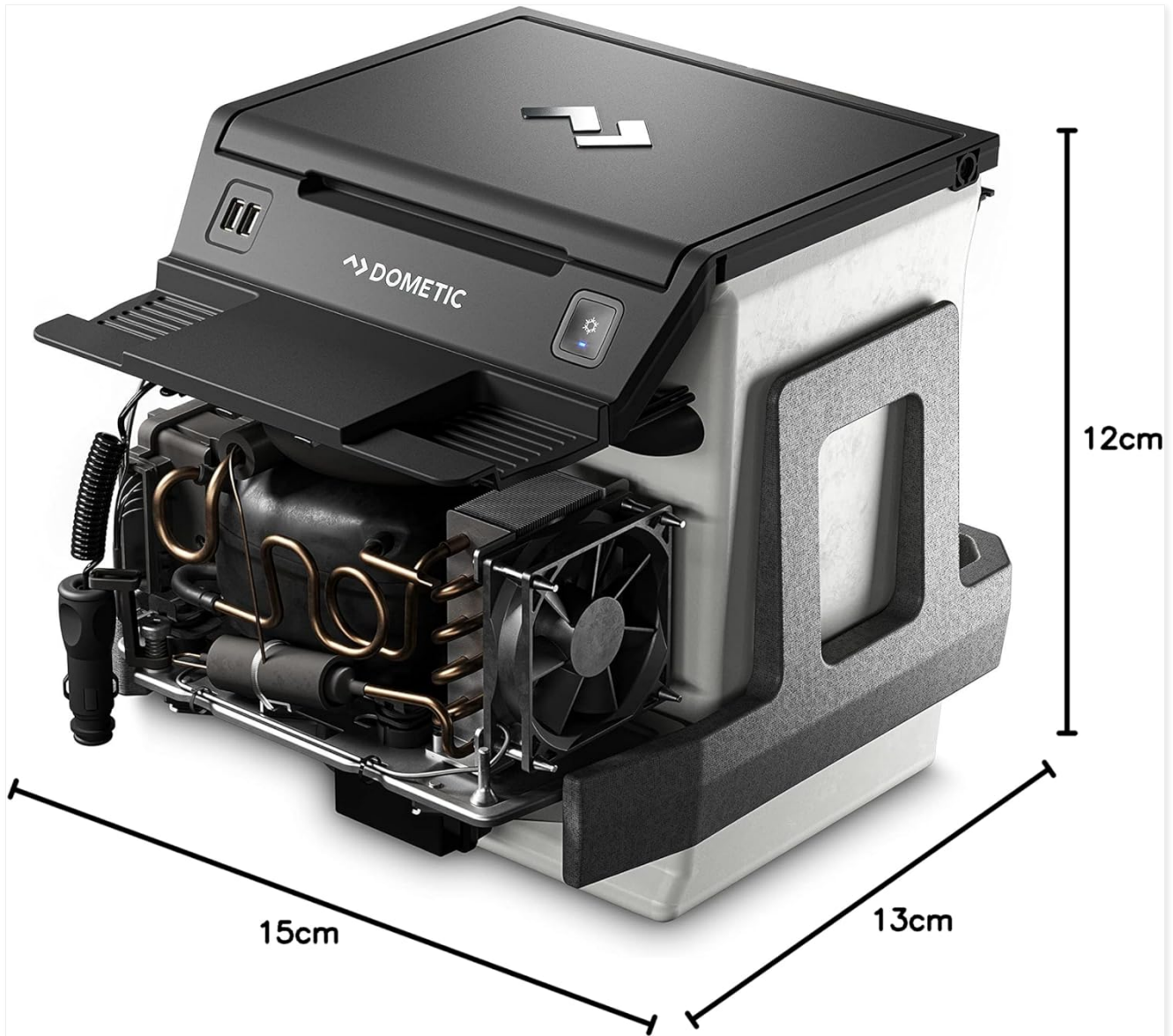
Figure 8.1: Dimensional overview of the Dometic CCF-T unit.
