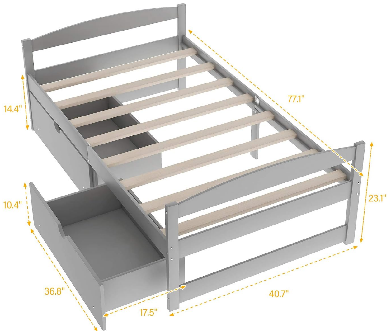
Figure 1: Overall Dimensions of the Twin Daybed and Storage Drawers.
