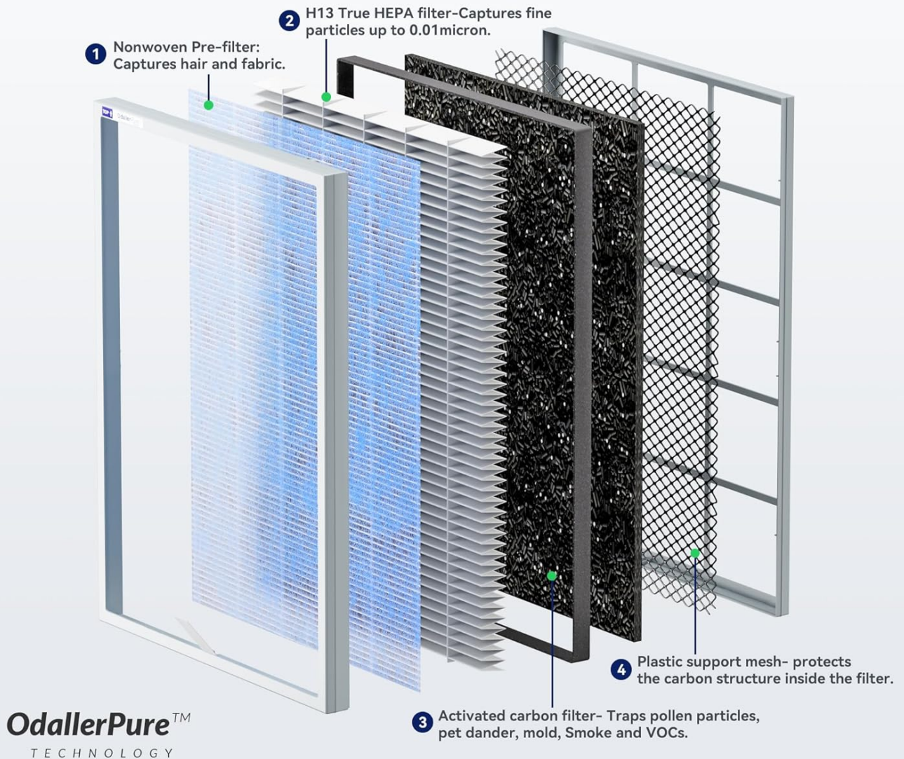
Image: A detailed diagram illustrating the 4 stages of filtration: Nonwoven Pre-filter, H13 True HEPA filter, Activated Carbon filter with OdallerPure™ Technology, and a plastic support mesh.
