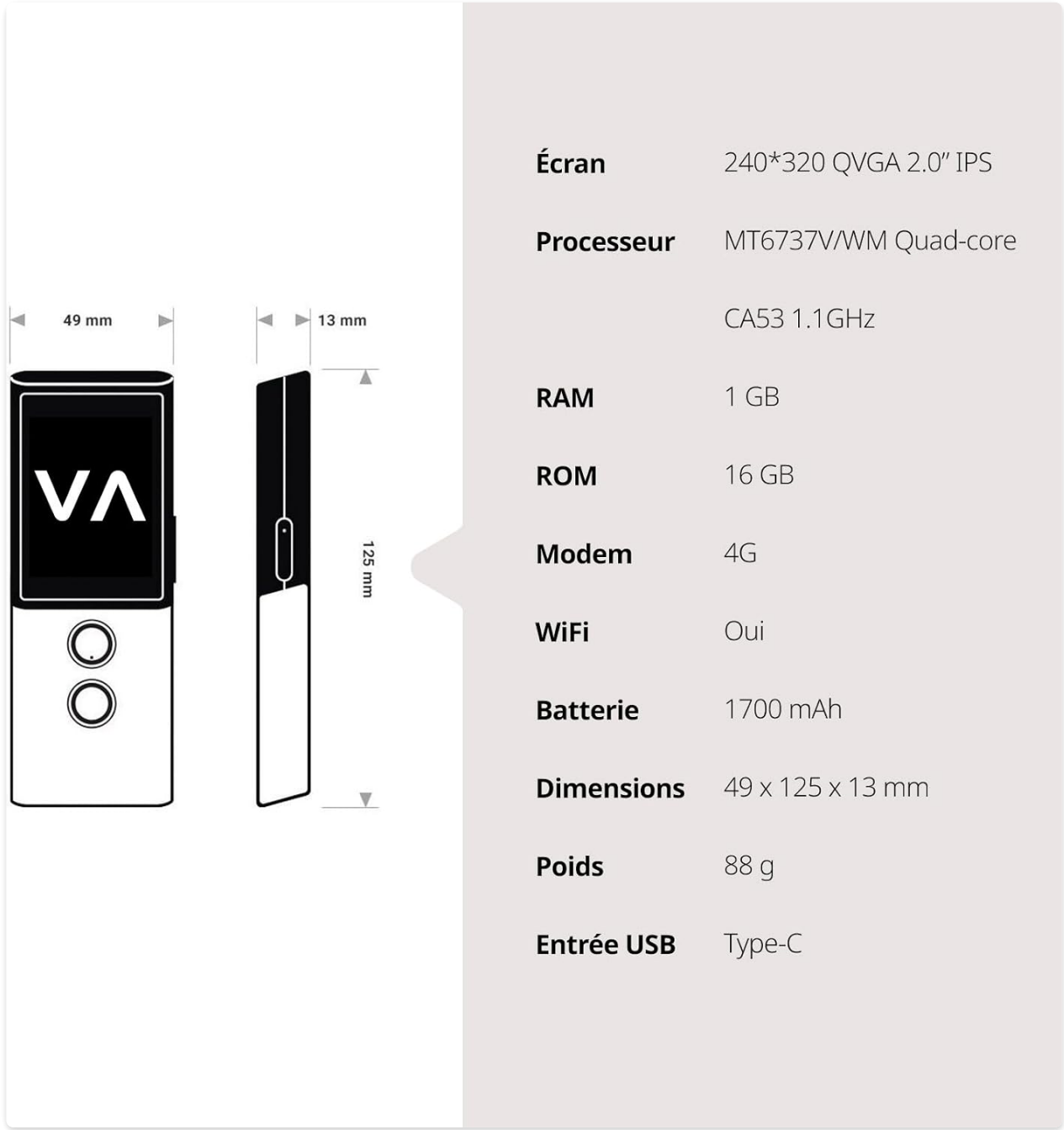
Figure 8: Technical specifications and dimensions of the Vasco Translator M3.
