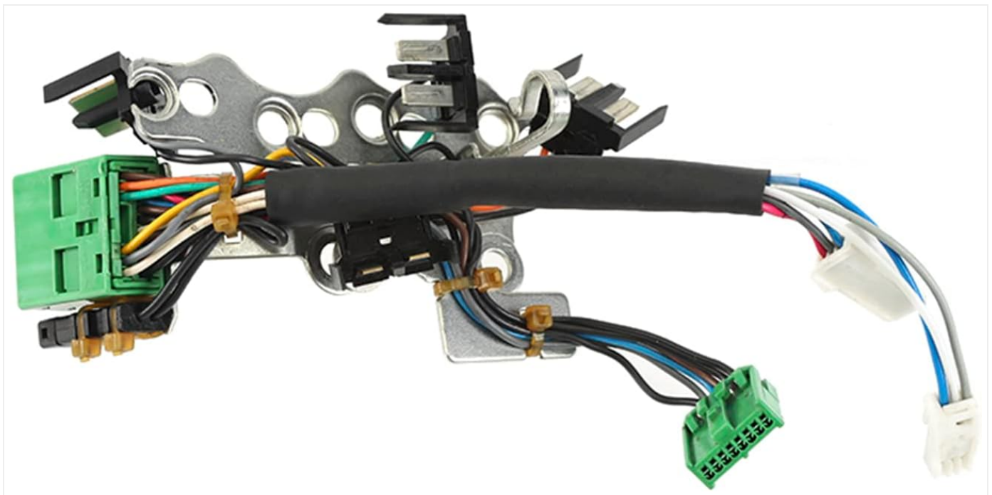
Image 2: Close-up of the JF011E Valve Body Wiring Harness. This image highlights the intricate wiring and connectors that integrate the solenoids into the transmission's control system.
