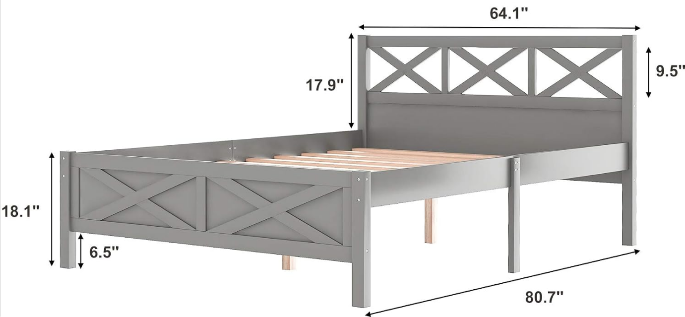
Figure 5: Illustrative dimensions of the platform bed frame. Refer to the table below for specific Full size measurements.
