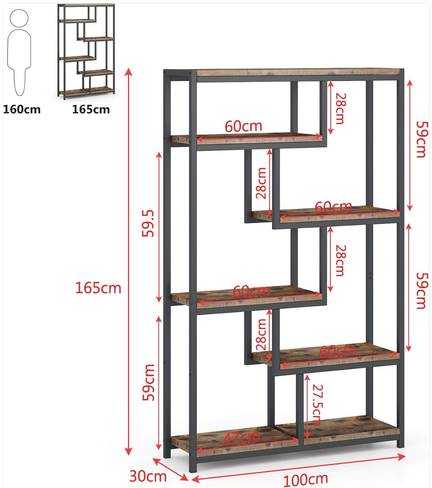
Image 2: A detailed diagram illustrating the dimensions of the Tribesigns 5-Tier Bookshelf, including height (165cm), width (100cm), and depth (30cm), along with individual shelf measurements.
