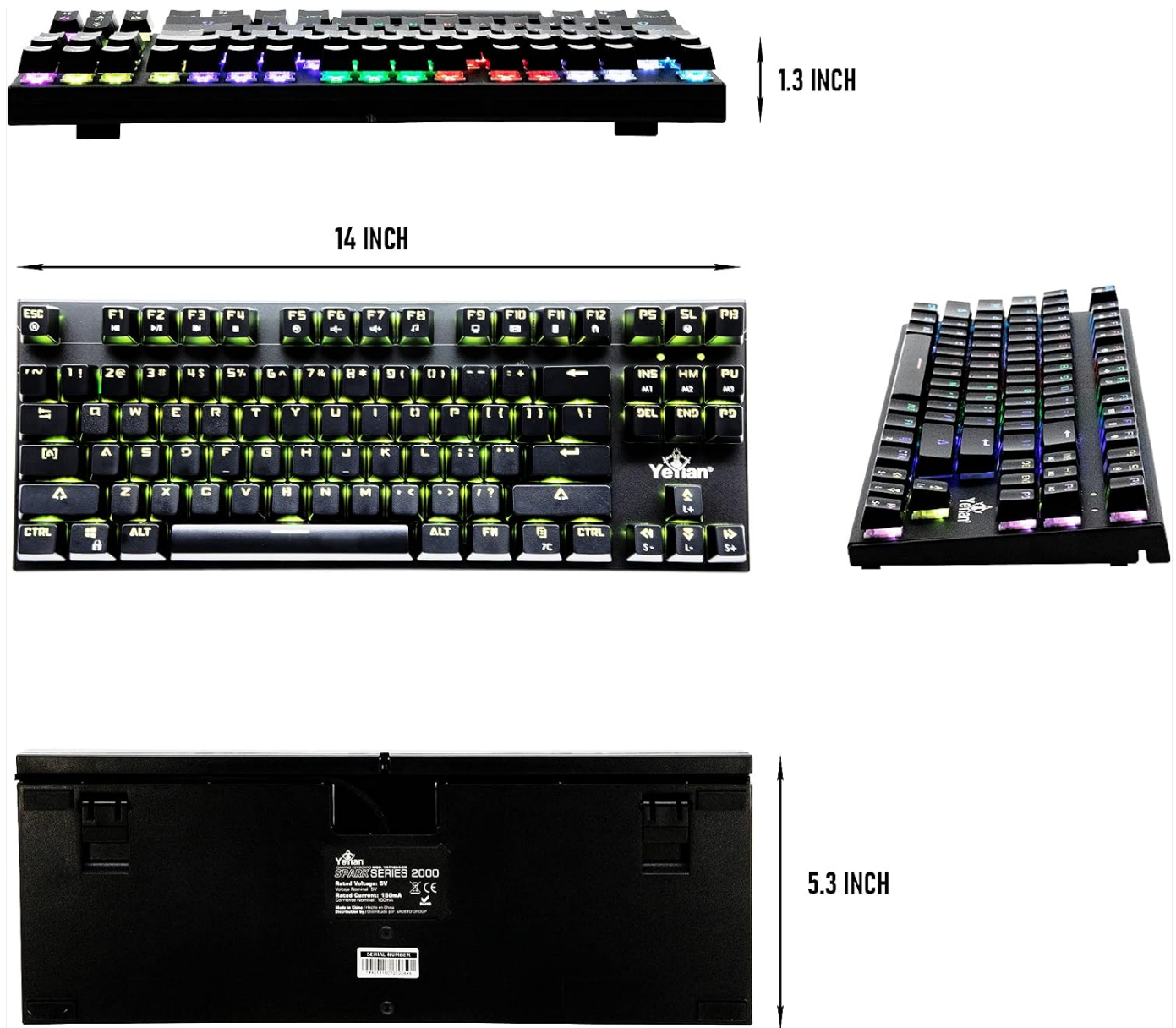
Image: Diagram illustrating the dimensions of the YEYIAN SPARK 2000 TKL keyboard.
