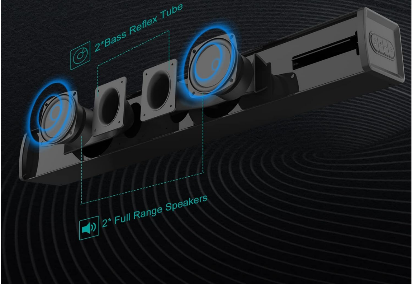
Image: Diagram showing the internal 2 full-range speakers and 2 bass reflex tubes of the 2.0 channel sound bar.
