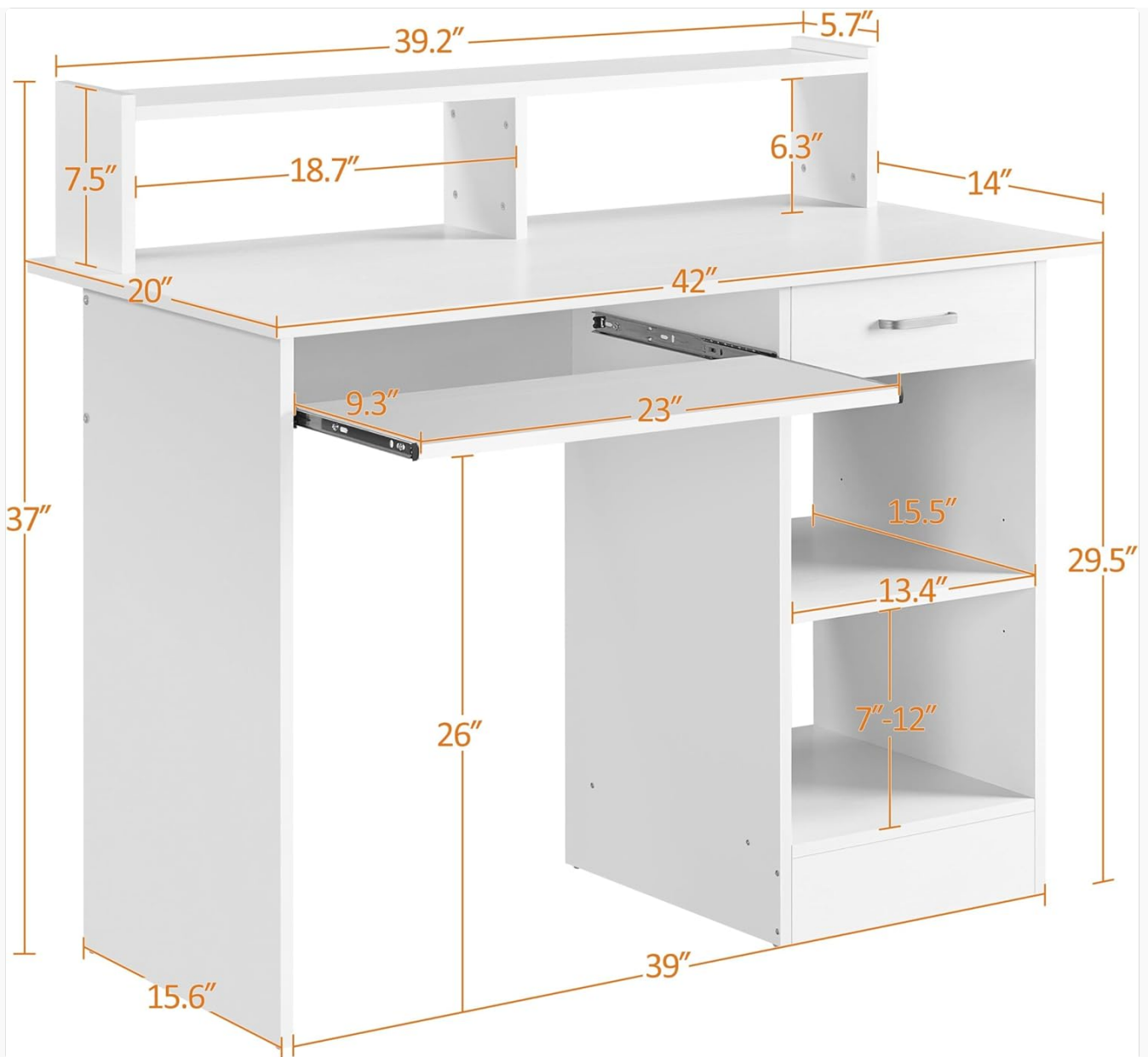
Image 7.1: Dimensional diagram of the Yaheetech Computer Desk, providing detailed measurements.
